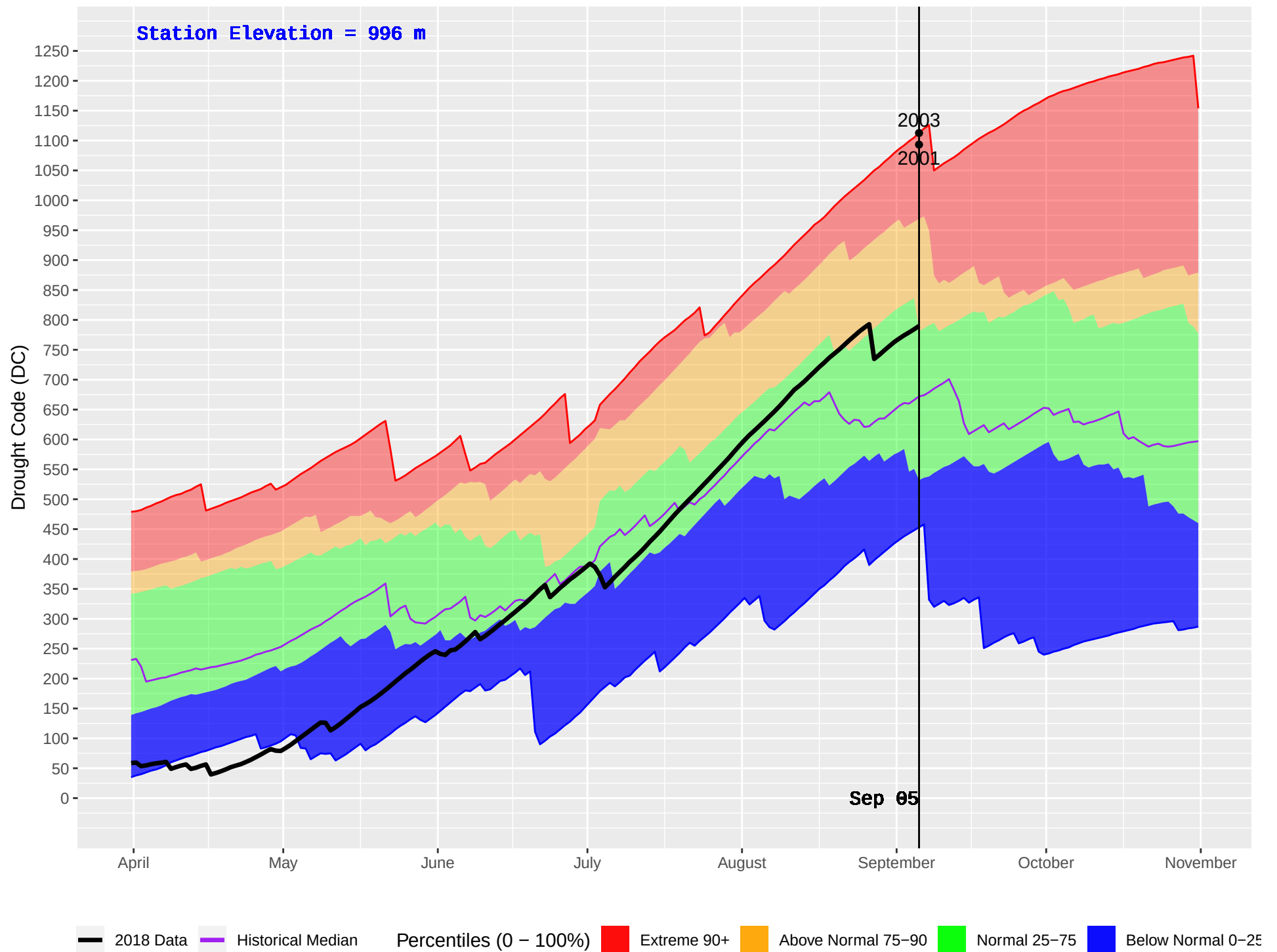
CRANBROOK FS (426) : Historical (2001–2016) and Current (2018) Daily Drought Code (DC)
