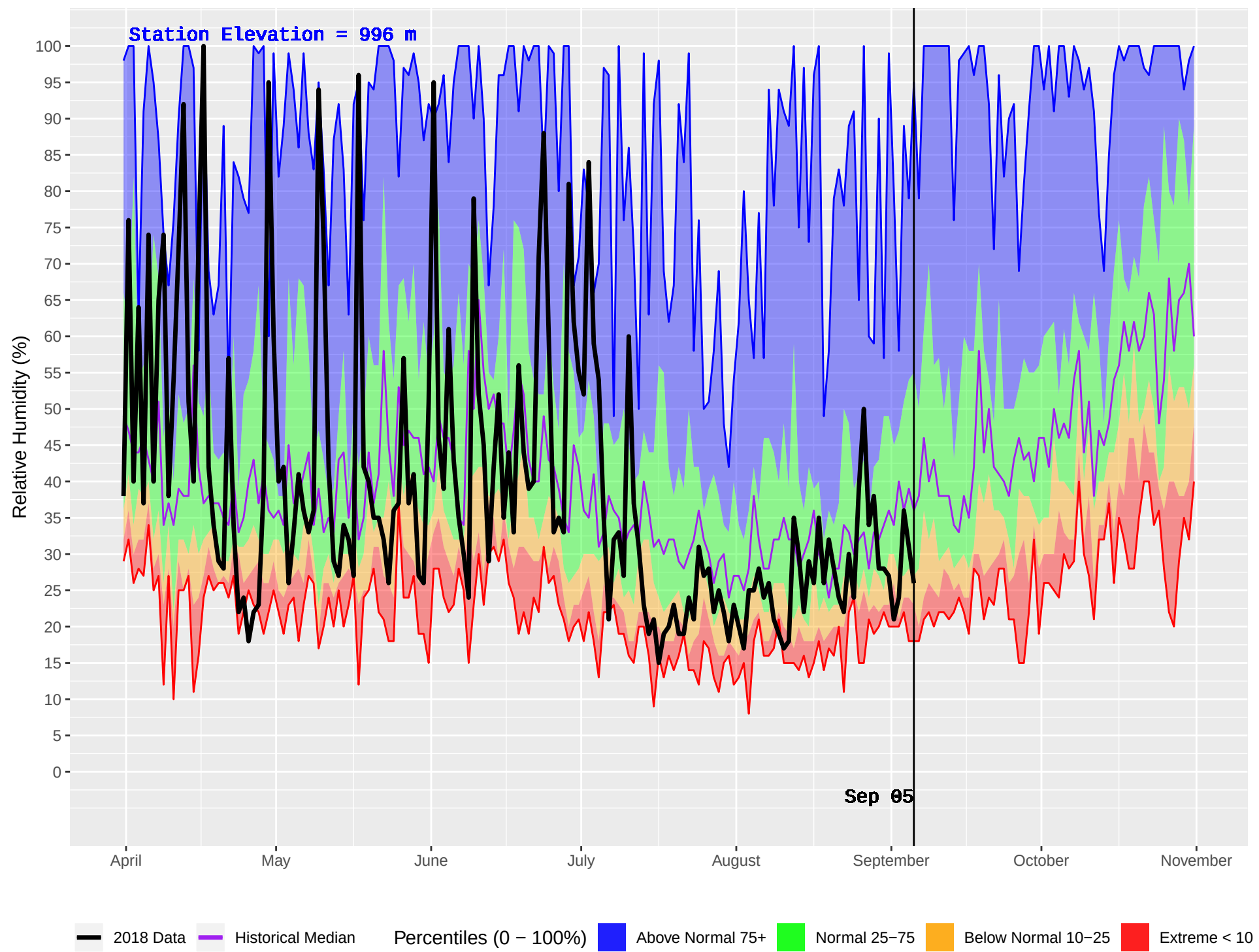
CRANBROOK FS (426) : Historical (2001–2016) and Current (2018) Daily Relative Humidity
