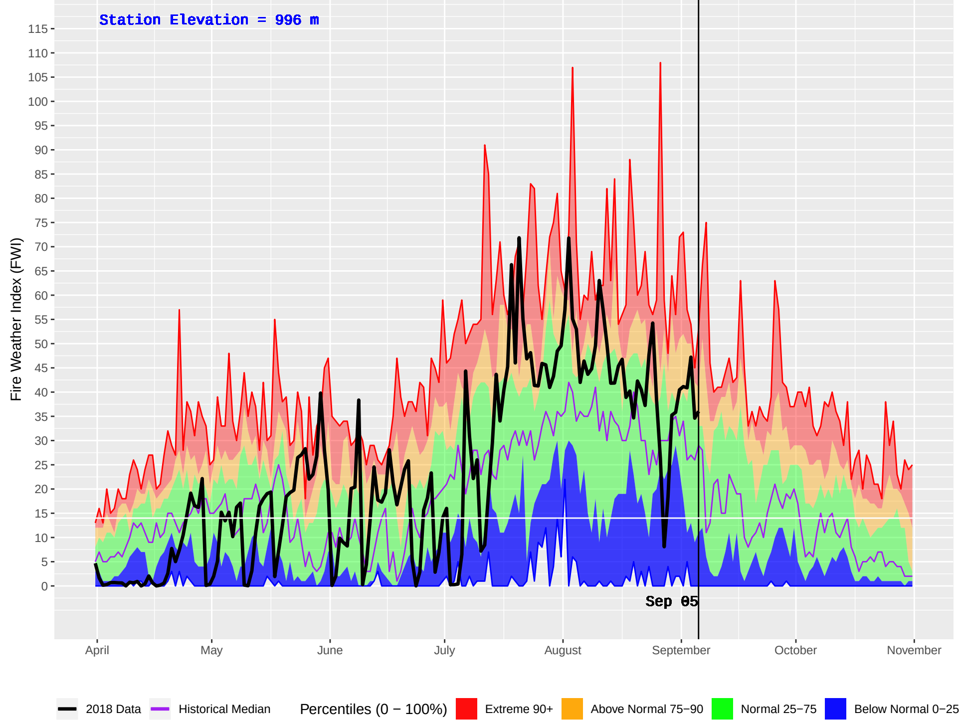
CRANBROOK FS (426) : Historical (2001–2016) and Current (2018) Daily Fire Weather Index (FWI)
