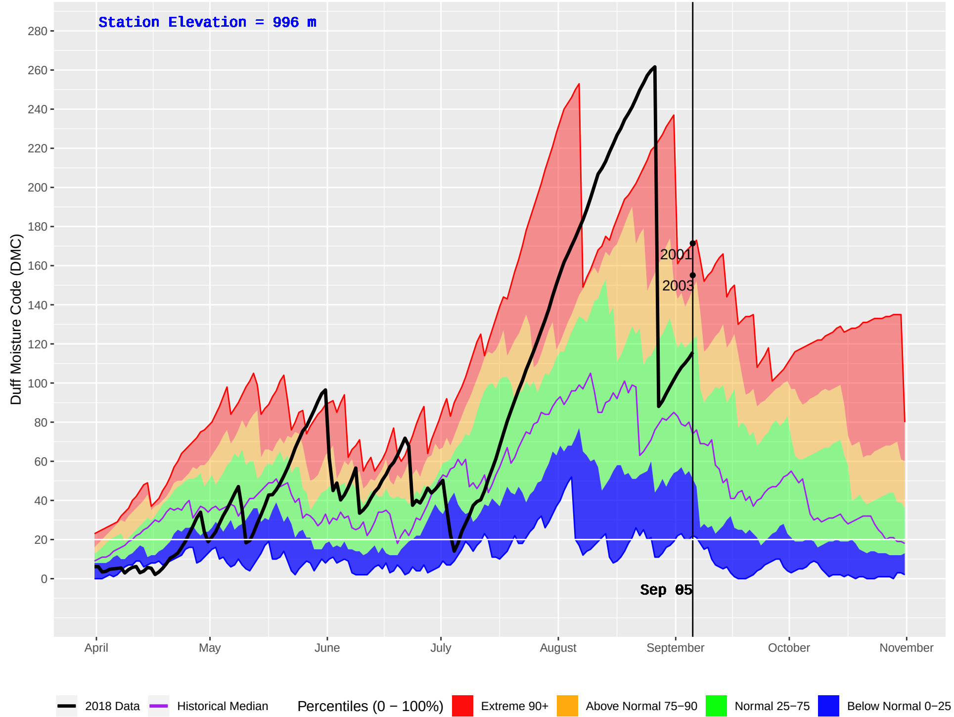
CRANBROOK FS (426) : Historical (2001–2016) and Current (2018) Daily Duff Moisture Code (DMC)
