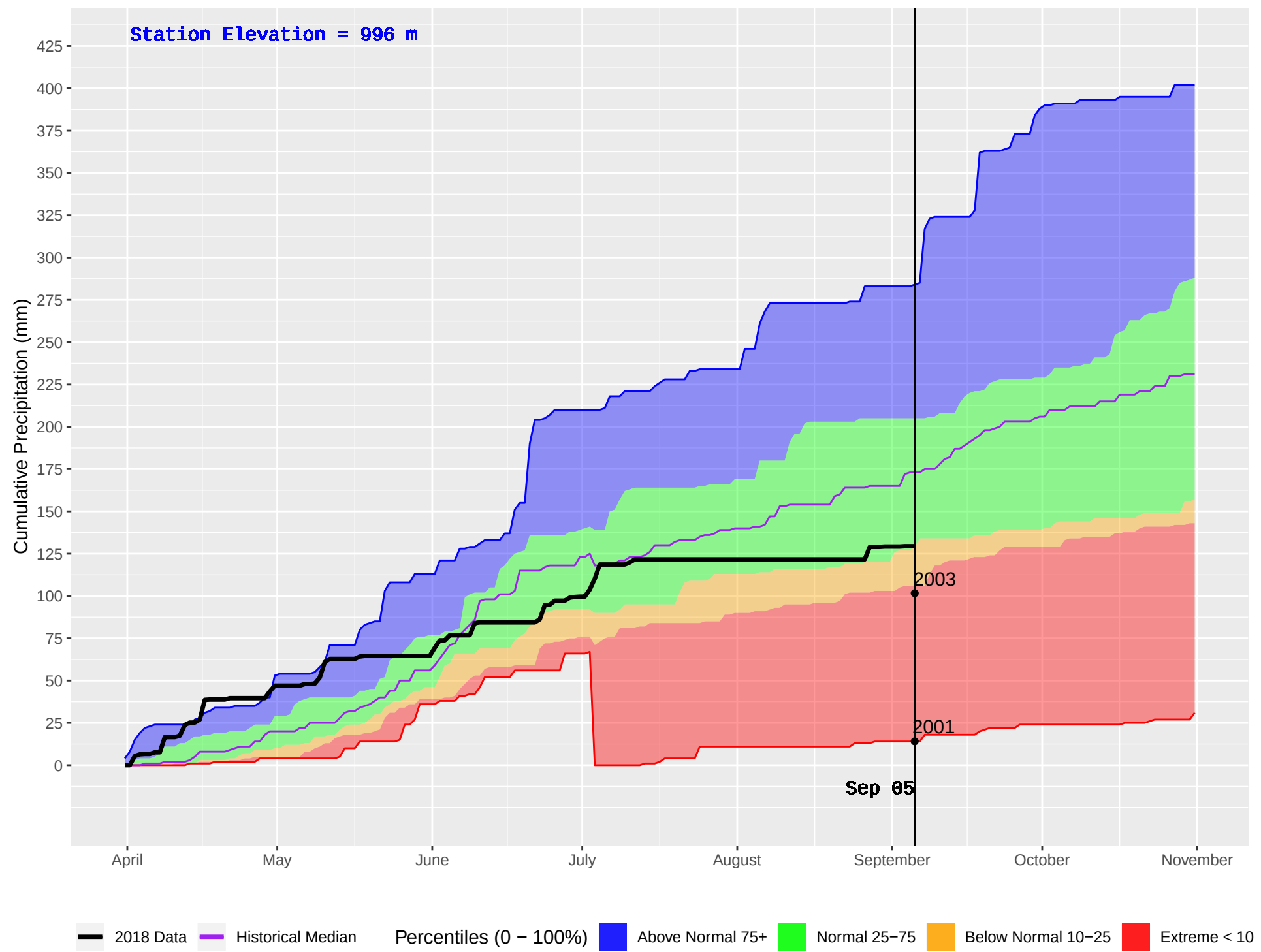
CRANBROOK FS (426) : Historical (2001–2016) and Current (2018) Daily Cumulative Precipitation
