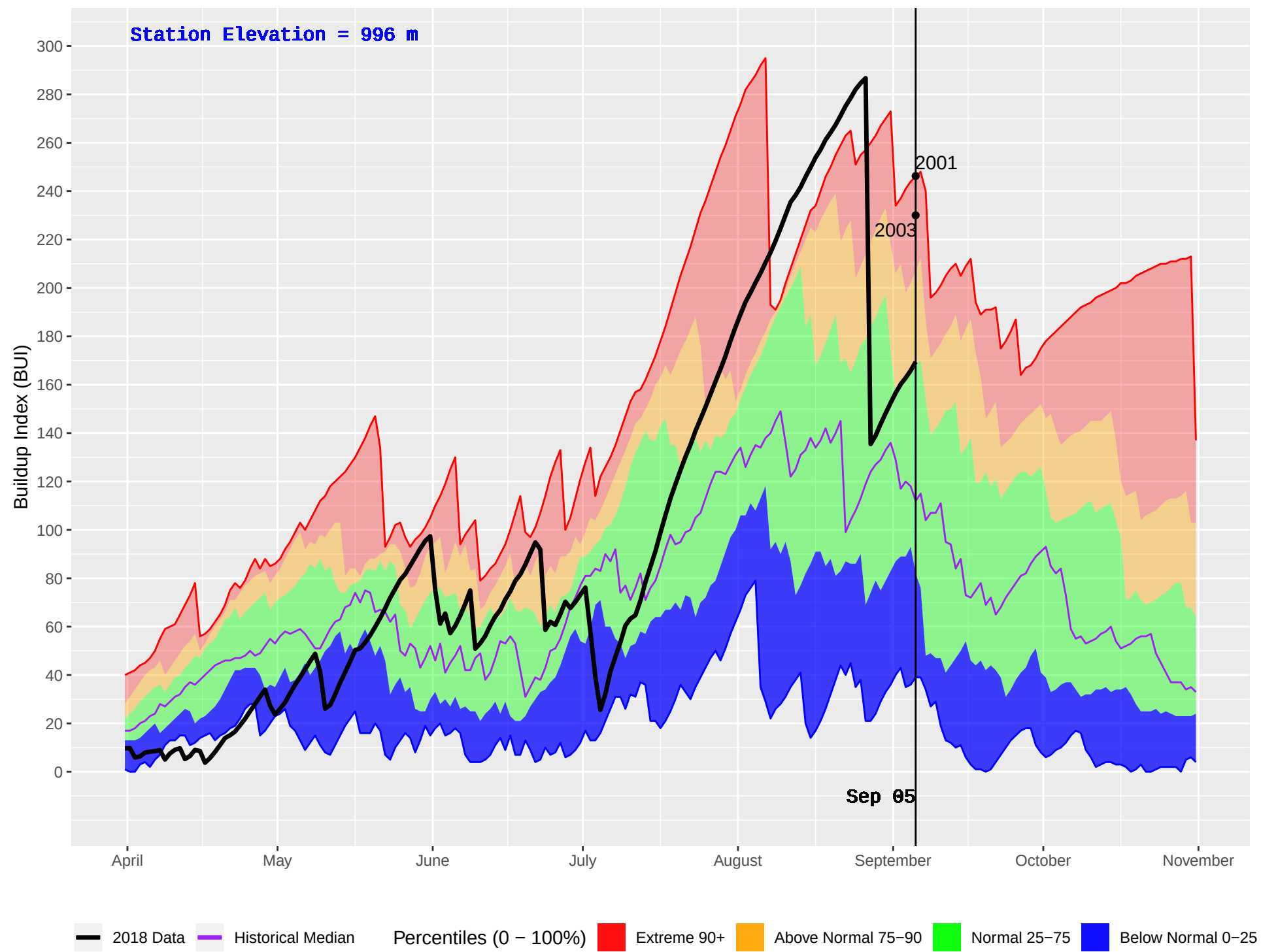
CRANBROOK FS (426) : Historical (2001–2016) and Current (2018) Daily Buildup Index (BUI)
