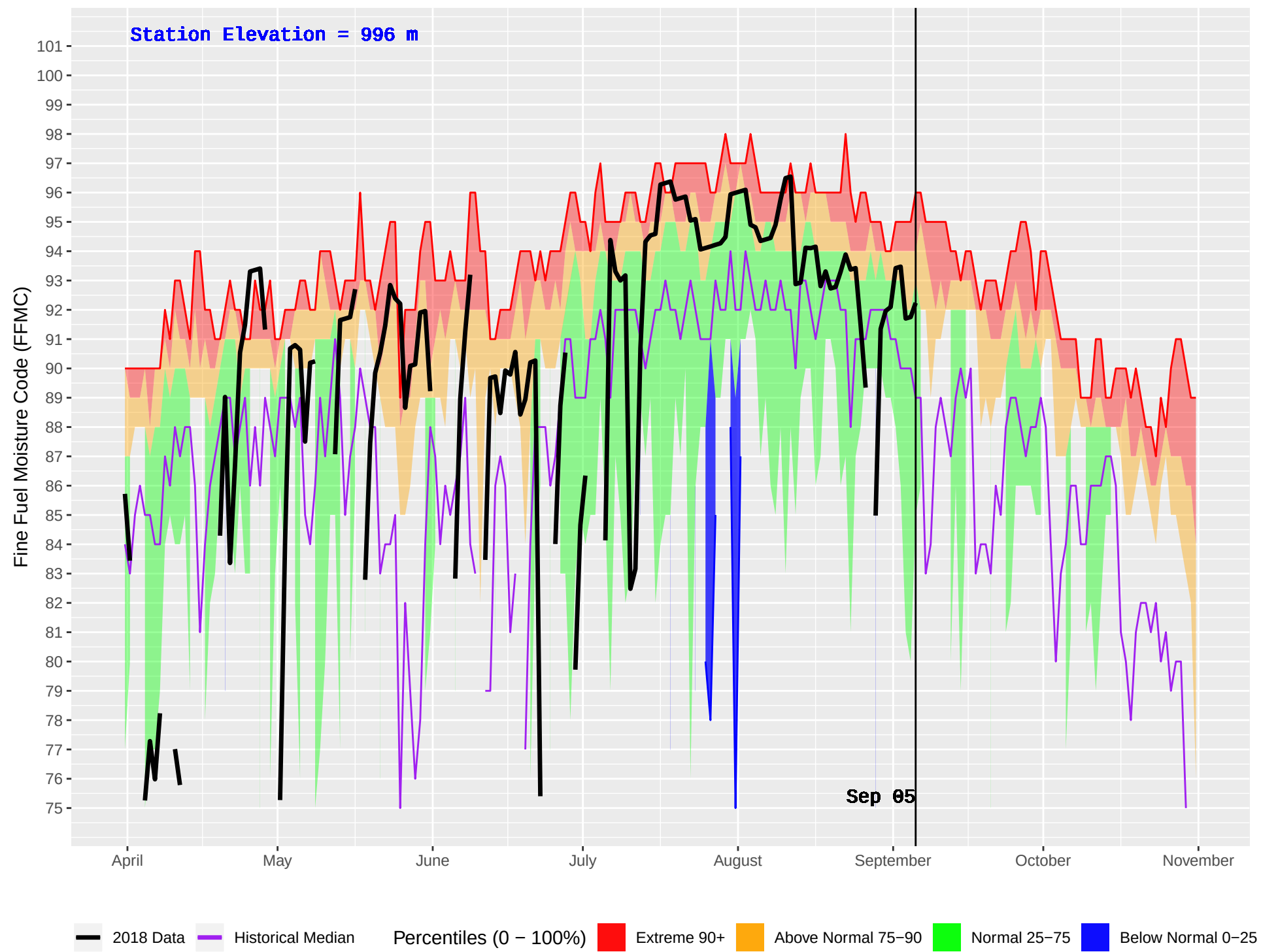
CRANBROOK FS (426) : Historical (2001–2016) and Current (2018) Daily Fine Fuel Moisture Code (FFMC)
